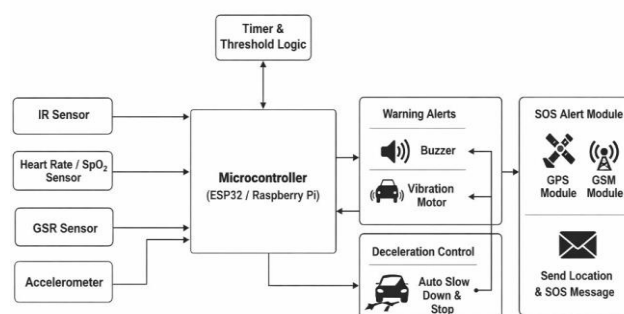
Fig. 1. Proposed timer based deceleration system with integrated SOS emergency
